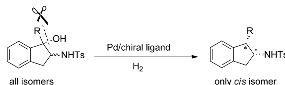
Scheme 1. Stereoconvergent palladium-catalyzed formal asymmetric hydrogenolysis of N -sulfonyl aminoalcohols.
